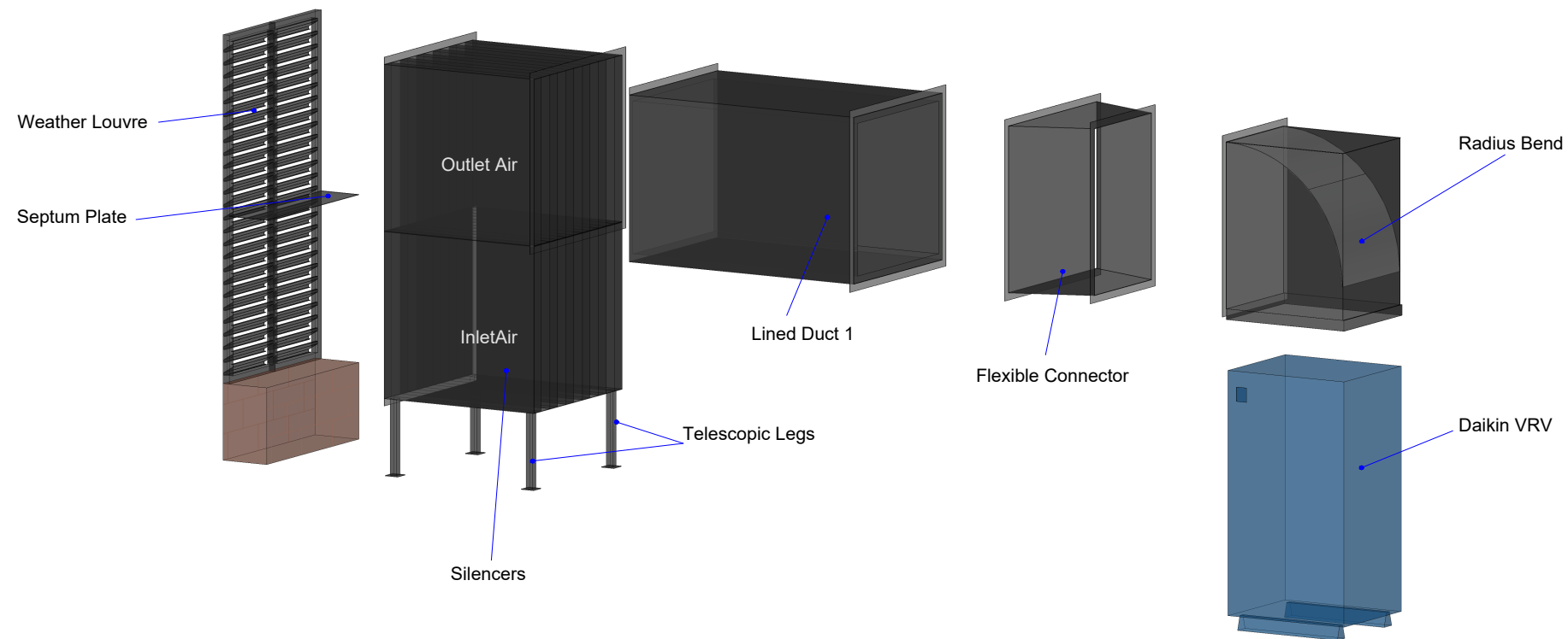
Expanded View
